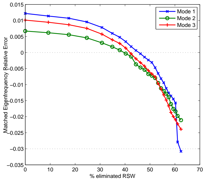
Figure 12: Results of optimization procedure for criterion 2 (threshold value = 2%) : eigenfrequency shift (reference = initial structure) versus number of removed RSW (reference = reinforced structure)
