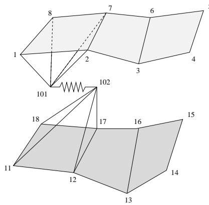
Figure 3: FE model of a RSW
