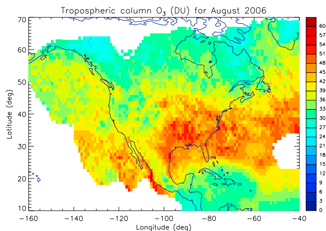
Figure 10. TOC field for August 2006 calculated by integrating the smoothed IONS-06 fields, like that shown in Figure 1 (bottom).
