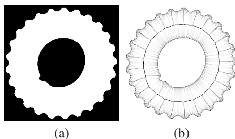
Figure 10.11. (a): a set X (in white); (b): the bisector function of X .
