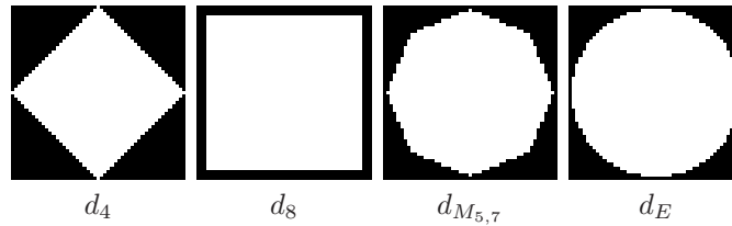
Figure 10.8. Discrete balls obtained from the d_4 , d_8 and d_{M_{5,7}} distances and from the Euclidean distance d_E
