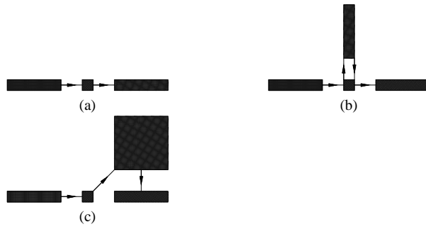
Fig. 1 (a) An arc \chi . The arrows give the ordering of the sequence. (b, c) Two elementary stretching of \chi .
