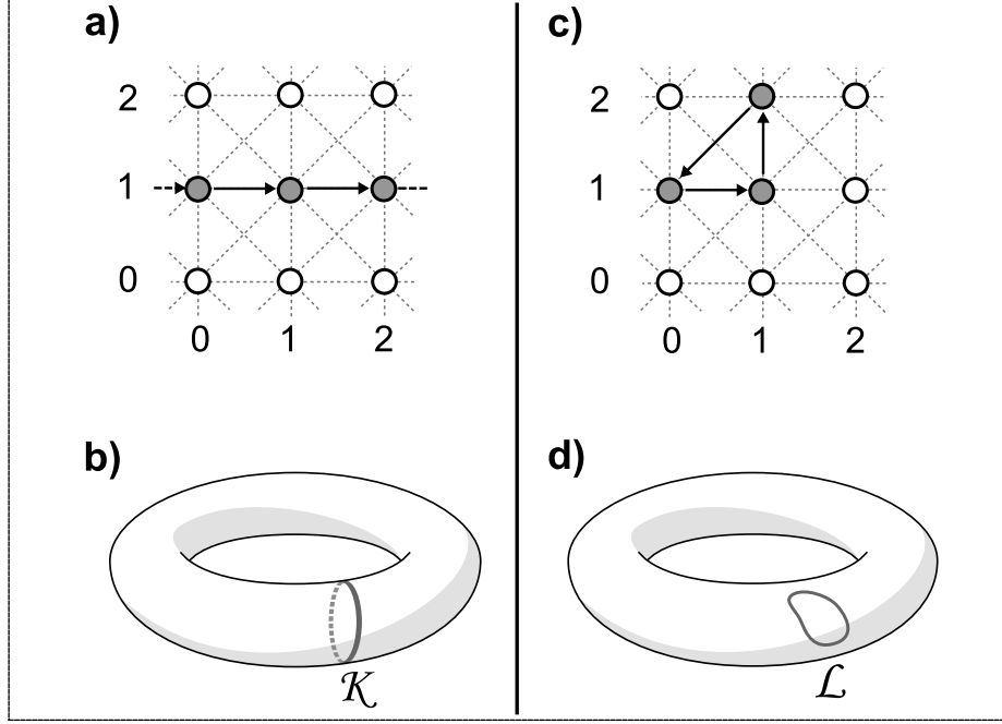
Fig. 8. Equivalent loops - In a and c : in \mathbb{T}^2 = \mathbb{Z}_3 \times \mathbb{Z}_3 , the loops in a ) and c ) are equivalent (see Def. 39) but not homotopic (see Def. 6). In b and d : the two loops do not belong to the same homotopy class in \mathbb{T}^2 , as one wraps around the toric space, and not the other.
