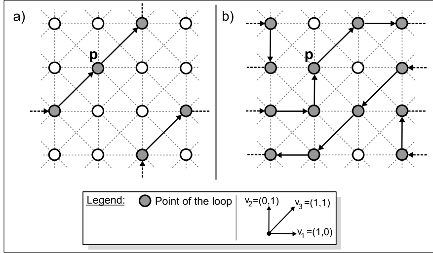
Fig. 5. Wrapping vector - In \mathbb{T}^2 = \mathbb{Z}_4 \times \mathbb{Z}_4 , the 2-loop in a) has a wrapping vector equal to (4, 4) , and the 2-loop in b) has a wrapping vector equal to (0, 0) .
