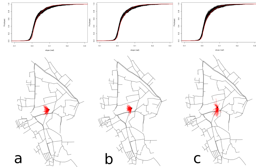
Figure 6: Similarity distribution of forests using a) r , b) f_2 , c) f_1 + f_2 . On the top, the F_\theta(slope) curves are depicted for the actual network (red) and the reconstructed networks (black). On the bottom, the Strahler barycenter of the actual network is depicted by the black point from which red segments join the reconstructed network Strahler barycenters.
