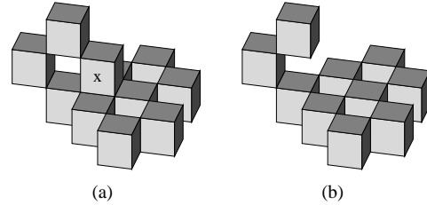
Figure 10. A lump made of 11 voxels is depicted in (a). It contains no simple voxel, and is simple-equivalent to the complex in (b), made of 10 voxels. Both objects have three tunnels.
