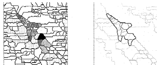
(c) Map of the basins valued by their dynamics (white = low, black = high)
