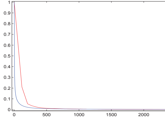
Figure 2: Normalized MAP criterion (Algorithm 4.1 in red and Algorithm 4.2 in blue) versus computational time (in seconds) (Intel Xeon 4 Core, 3.00 GHz).
