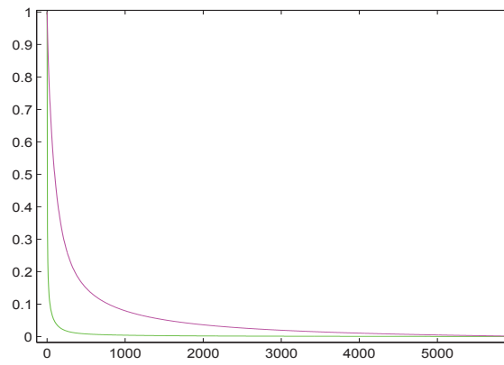
Figure 3: Normalized MAP criterion (for \theta = 0.25 in green and \theta = 10 in magenta) versus computational time (in seconds) (Intel Xeon 4 Core, 3.00 GHz).
