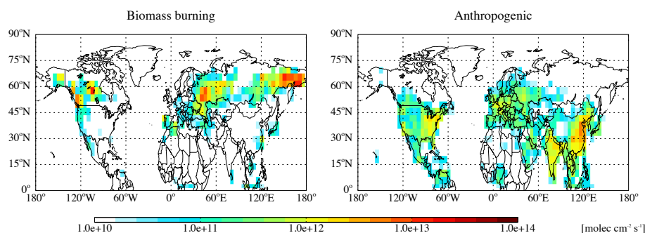
Fig. 10. Mean Northern Hemisphere CO emissions from biomass burning and anthropogenic sources ( \text{molecules cm}^{-2} \text{s}^{-1} ) averaged over 12 July to 4 August 2010. Biomass burning emissions are from the FLAMBE inventory (Reid et al., 2009). Anthropogenic emissions in the model are as those described in Sect. 3.
