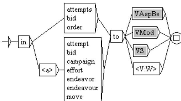
Figure 1: “In order to + verb” graph
