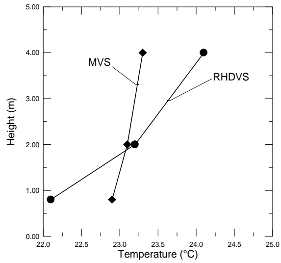
Figure 10 - Vertical temperature gradient (RHDVS and MVS comparison).
