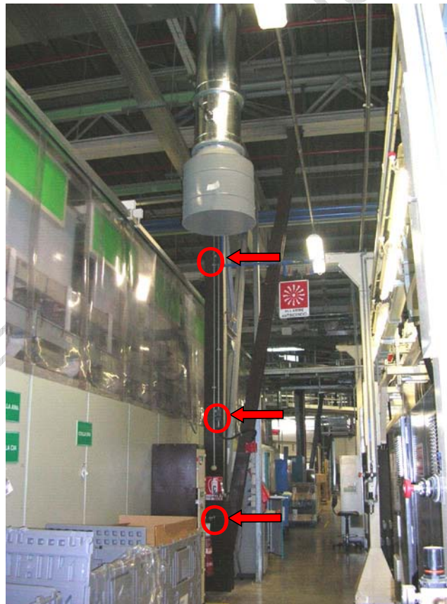
Figure 11 - Temperature sensors location and RHDVS test diffuser.
