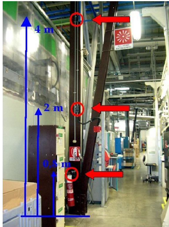
Figure 8 - Temperature sensors location.
