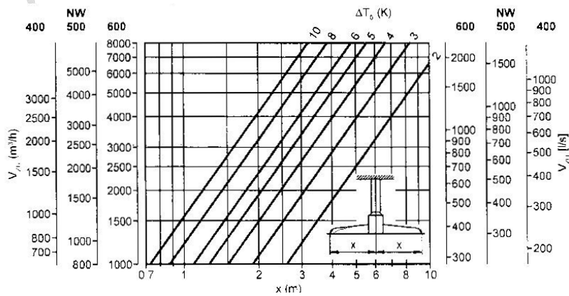
Figure 3 - Typical flow characteristics of diffuser with horizontal air ejection (NW = Diffuser diameter in mm).
