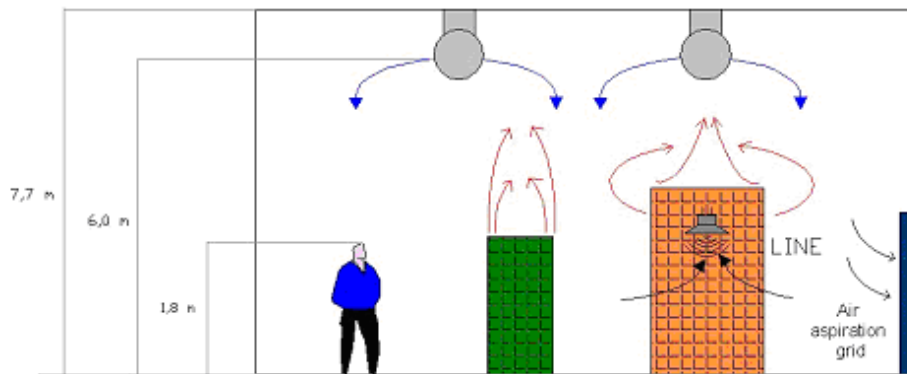
Figure 1 - Scheme of mixing ventilation system.
