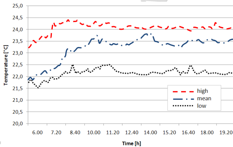
Figure 13 - Temperature readings (RHDVS).
