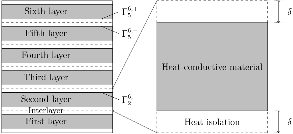
Figure 3: The multilayer geometry, six layers: N = 6 .
