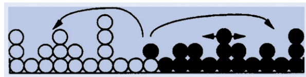
Figure 1. Illustration of the Bak, Paczuski and Shubik model: white particles (buy orders, bid) moving from the left, black particles (sell orders, ask) moving from the right. Reproduced from Bak et al. (1997).
