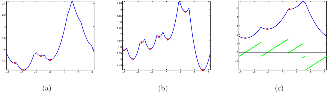
Figure 4: (a) and (b) Plots of F_{\mu^n} where n = 10 and \mu^n = \sum_{i=1}^n \delta_{X_i} where the X_i i.i.d of uniform law \lambda . The red points are the local minima computed with the described algorithm. (c) In blue: plot of F_{\mu^n} where n = 4 . In green: the derivative of F_{\mu^n} . The critical points are given by the intersection between the green curve and the x -axis in black.
