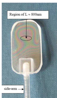
Figure 1: Photography of the NTC. Since NTC gap thickness is of order of visible light wavelength, interferometric pattern occurs. Region of L = \lambda = 800 nm is indicated, NTC has a sapphire side-arm.
