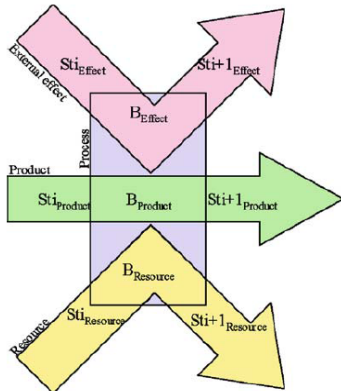
Figure 7: FBS-PPRE model [30].
