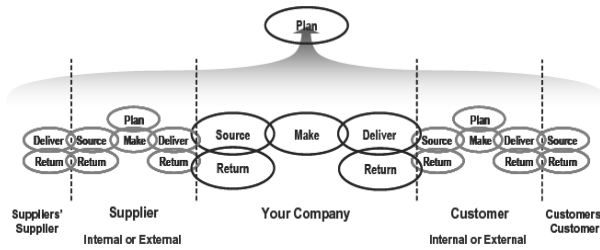
Figure 9: SCOR model [39]
