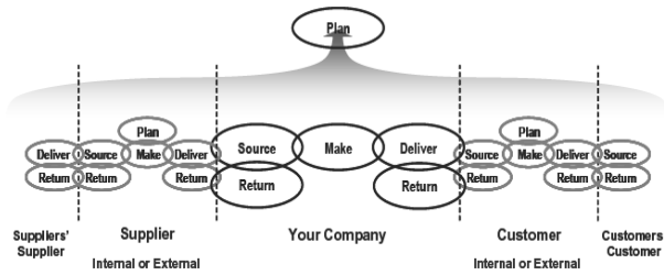
Figure 9: SCOR model [39]
