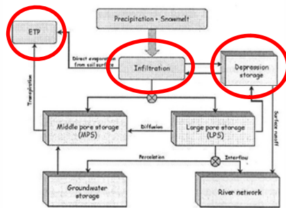
Fig. 1. The concept of the soil-water module of the J2000, showing the storages and processes. Krause, 2002
