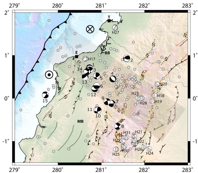
Figure 7. Upper plate deformation and events locations from ESERALDAS experiment (gray circles) and GCMT catalog data. Focal mechanisms are lower hemisphere projection (black compressional quadrants = ESERALDAS solutions; gray compressional quadrants = GCMT solutions). Neotectonic structures are from Eguez et al. [2003]. Gray stripe underlines denser seismic activity, coinciding with the limit between a northern subsident segment and a southern uplifted segment. MB = Manabí Basin; BB = Borbón Basin; E = Esmeraldas city and T = Tumbaco city.
