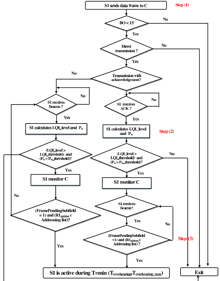
Fig. 3. The global flowchart of muDog
