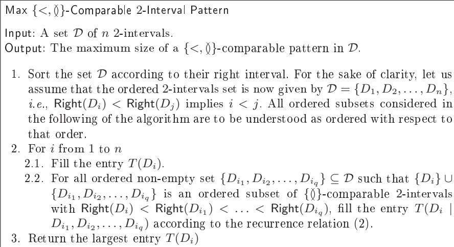
Fig. 2. Algorithm Max \{<, \emptyset\} -Comparable 2-Interval Pattern.
