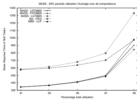
Figure 5. MASS, 90% load
