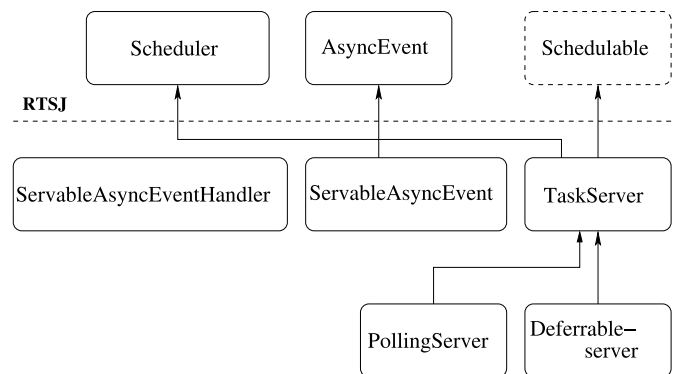
Figure 1. Classes to implement the server policies
