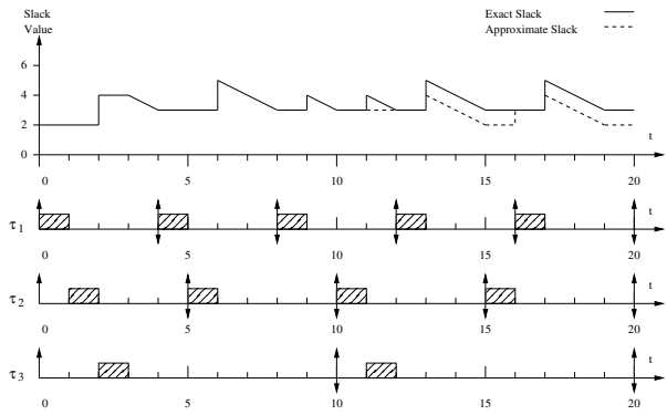
Figure 3. A system of 3 tasks with the associated slack at each instant.
