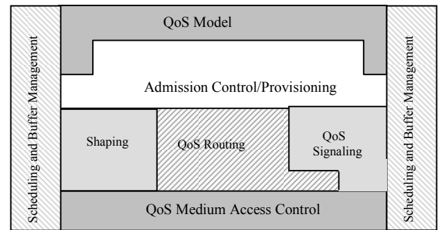
Fig.5. QoS Components
