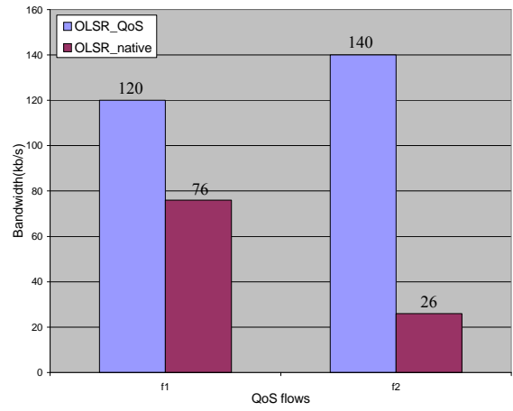
Fig.13. Average measured bandwidth with QoS support and native OLSR
