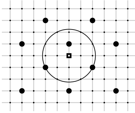
Figure 1: An optimal identifying code for \mathbb{Z}^2 (from [9]) with Euclidean radius r = \sqrt{5} .
