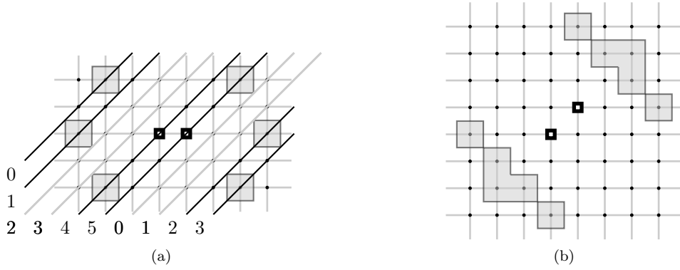
Figure 4: In (a), the set \mathcal{S}_{3,\sqrt{10}-3}((0,0),(-1,0)) is intersecting all the diagonal and anti-diagonal lines modulo 6. In (b), the set \mathcal{S}_{3,\sqrt{10}-3}((0,0),(-1,-1)) is intersecting all the horizontal and vertical lines modulo 8.
