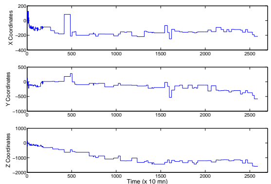
Figure 1: Typical Variations of a node’s coordinate in the Vivaldi System.
