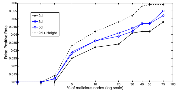
Figure 11: Self Isolation: False Positive Ratio.
