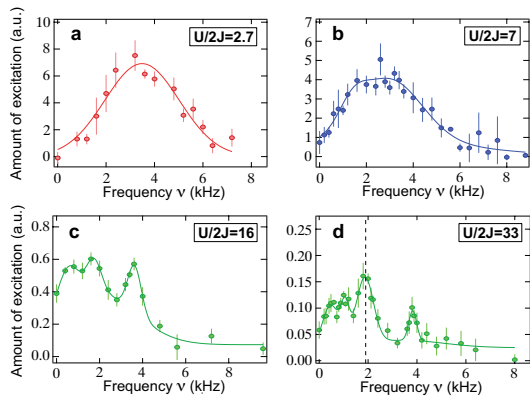
FIG. 2. Bragg spectra of the 1D gases across the superfluid to Mott insulator transition for four ratios U/2J along the axis of the 1D atom tubes: 2.7 (corresponding to s_y = 4 ), 7 ( s_y = 7 ), 16 ( s_y = 10 ) and 33 ( s_y = 13 ). The solid lines are guide to the eye. The vertical dashed line in d) marks the particle-hole excitation energy \Delta_{p-h}(q_0) . (Color online)
