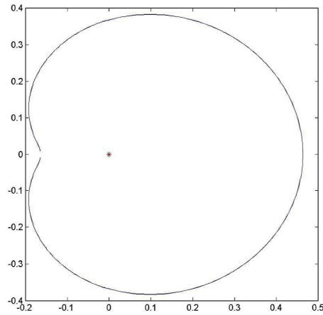
FIGURE 3. Internal boundary \partial B for g_0 = 1 and g_1 = 0, 13668 > g_{cr}
