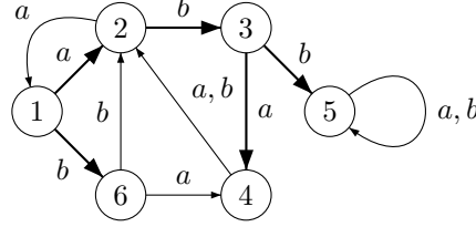
Fig. 2: A transition structure on a 2-letter alphabet having 1 as initial state
