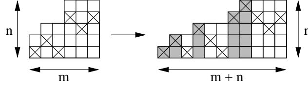
Fig. 4: From a boxed diagram to the set partition \{\{1, 3, 6\}, \{2, 5\}, \{4, 10\}, \{7, 9, 11\}, \{8\}\}
