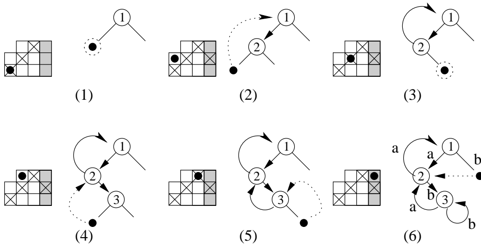
Fig. 3: From a 2-Dyck boxed diagram B' to a transition structure of \mathcal{D}_n
