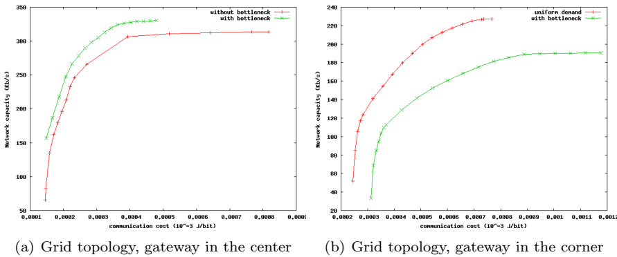
Figure 21: Capacity and energy tradeoff, assuming Idle cost = 0, with power control.
