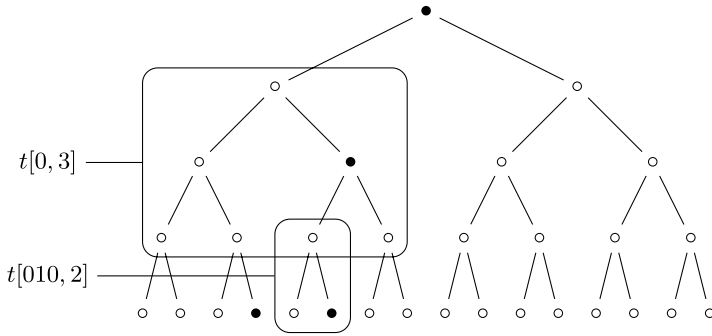
Fig. 2 The top of the Dyck tree of Example 1 and two of its factors, of height 3 and 2, respectively. Again, a is represented by ● and b by ○
