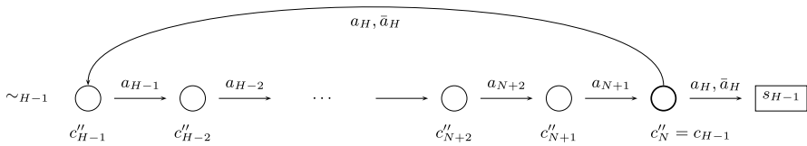
Fig. 23 The irrational classes of \sim_{H-1}
