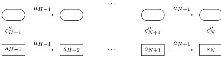
Fig. 20 The classes of \sim_{H-1} . The classes c''_N, c''_{N+1}, \dots, c''_{H-1} are irrational, and the (rational) classes containing the states s_N, s_{N+1}, \dots, s_{H-1} are singletons
