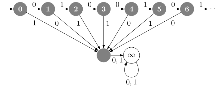
Fig. 9 Automaton of the band indicator tree of width 1 for the Fibonacci word 01001010... . Only one state is not final
