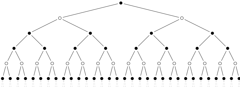
Fig. 1 The top of a uniform tree for the word abaaba . . . . Node label a is represented by ●, and label b is represented by ○. This tree will be seen to have infinite degree and rank 0
