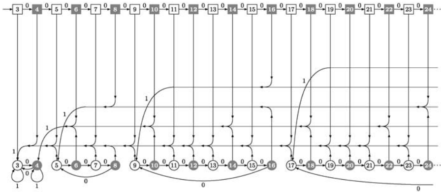
Fig. 25 Final states are dark. Observe the fractal-like structure, with a doubling of the size of each block
