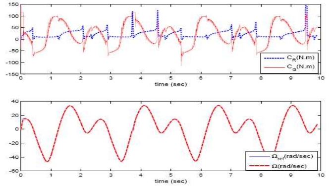
Fig. 14. Kite applied torque ( C_R ), Generator Torque ( C_G ) and Rotation velocity tracking for orbit 3.
