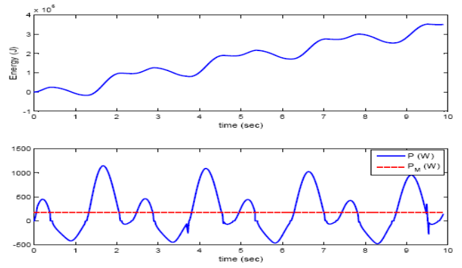
Fig. 13. Orbit 3's Power Generation, P_M mean power.
