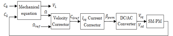
Fig. 5. Converter control Diagram.
