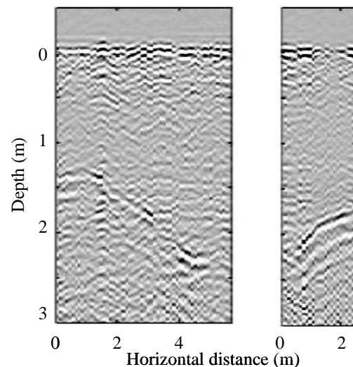
Fig.2 : Example of two perpendicular profiles showing the same buried interface between 1.5 and 2.5 meters below the surface.
