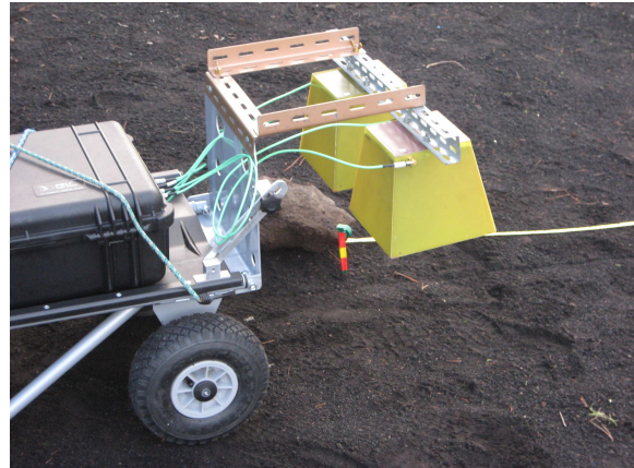
Fig. 1 : WISDOM prototype on Mount Etna
