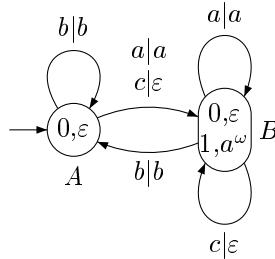
Figure 6: Transducer \mathcal{S} of Example 17
