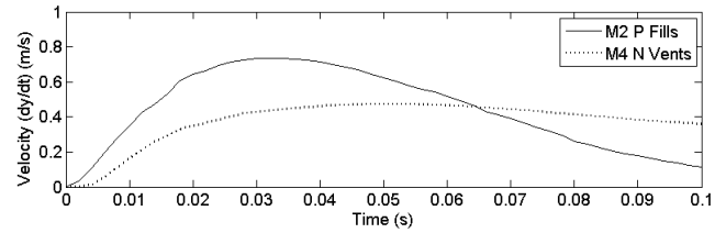
Fig. 3. Open-loop responses modes M_2 and M_4
