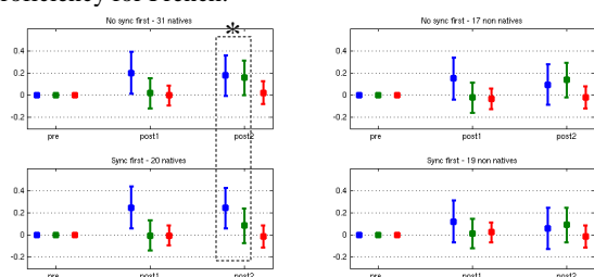
Figure 5. Relative improvement in orthographic quiz score after using each system (bottom synchronous reading first; top: second) in comparison with the pretest for native (left) vs. non native (right) readers. For each of the three quiz, the performance is given for three sets of words from left to right: the 10 words read by system A, the 10 words read by system B and the remaining 20 words of each quiz never read. Significant contrasts ( p < 0.1 ) are cued by stars.
