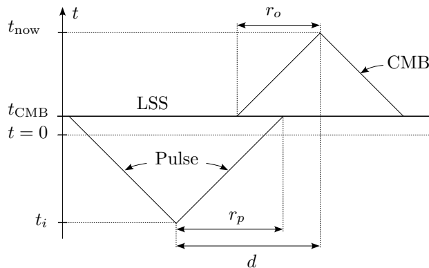
FIG. 1: The conformal diagram of the expanding (null) pulse, intersecting the last scattering surface (LSS). The CMB sphere as seen today is also pictured. The time t = 0 corresponds to the transition between the pre-big-bang and post-big-bang epochs. The detailed dynamics near the transition point are of course model-specific.
