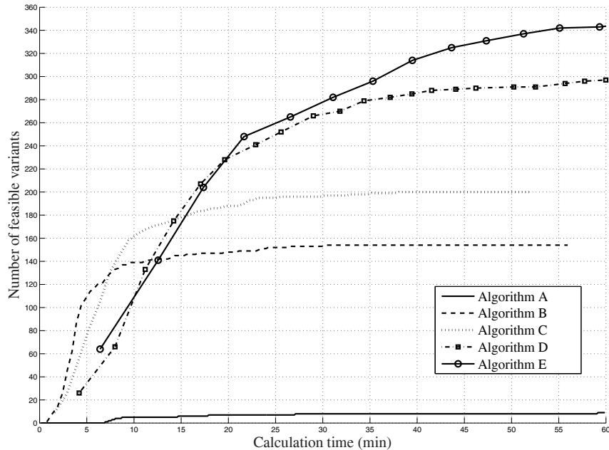
FIGURE 6. COMPARISON OF THE OPTIMIZATION ALGORITHMS.
