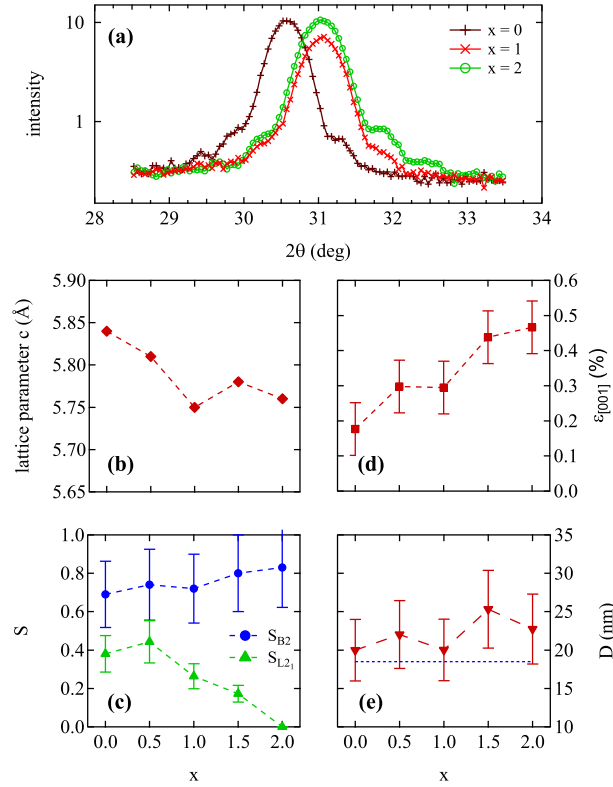
Figure 1. (a): \theta - 2\theta scans of the (002) reflections of Mn_2 VAI ( x = 0 ), Mn_1Co_1 VAI ( x = 1 ), and Co_2 VAI ( x = 2 ). Clear Laue oscillations are visible in both cases. (b): out-of-plane lattice parameter c as function of x . (c): Order parameters S_{B2} and S_{L21} as functions of x . (d): Microstrain \varepsilon_{[001]} and (e): coherence length D and as functions of x . The dashed line in (e) denotes the film thickness.
