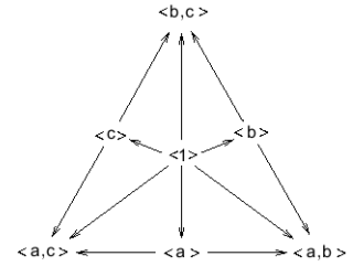
FIGURE 1. Quotient of the Davis complex for a triangle group (diagram reprinted with the kind permission of Sanchez-Garcia [25]).
