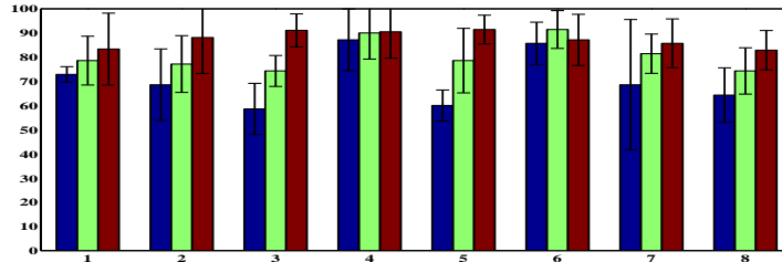
Fig. 2: Performances of classical SVM (Left bar), sw-SVM (Middle bar) and proposed method (Right bar) for the 8 subjects. Mean (std) accuracies across the 8 subjects were 70.71(10.77), 80.71(6.61) and 87.51(3.37) respectively.
