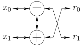
Fig. 2: Simplified bipartite graph of the (4,2,2) Hadamard code.
