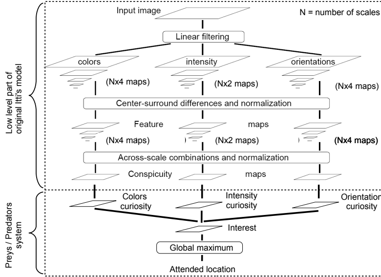
Fig. 1. Architecture of our bottom-up visual attention model. This diagram has been adapted from [5].
