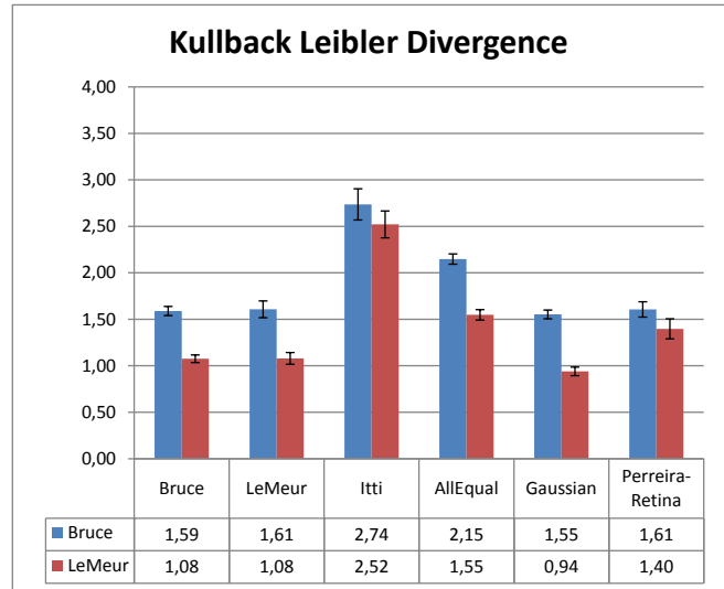
Fig. 4. Comparison to ground-truth : comparison of different algorithms. (Please note that for KLD, lower values mean more plausibility),
