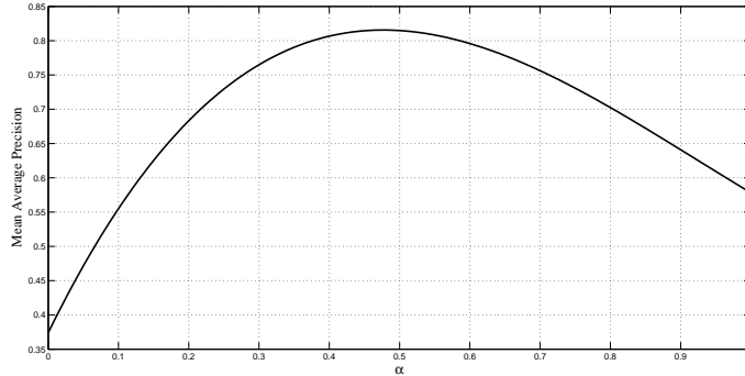
Figure 11: Impact of \alpha on the average precision. Fifteen points were computed and the curve has been interpolated using a 3rd order function.
