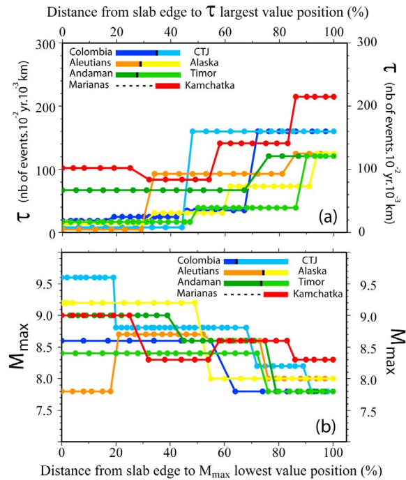
Figure 13. Along-trench variations of (a) seismic rate \tau and (b) M_{max} . Along-trench variations are plotted for half-trench systems. For each half-trench system, distances are expressed as percentages of the distance between the slab edge and the largest \tau value position (Figure 13a) or the lowest M_{max} value position (Figure 13b). Black marks on the insets indicate the along-trench position of the largest \tau value (Figure 13a) and the lowest M_{max} value (Figure 13b) for each trench system. Variations are plotted from the slab lateral edges, where the lowest \tau and largest M_{max} values are located, toward the largest \tau and lowest M_{max} positions, which are located in the vicinity of the geographical centers of the trench system. Trench systems are as follows: blue, South America (Colombia and Chilean Triple Junction (CTJ) edges); orange, Aleutians-Alaska (western Aleutians and eastern Alaska edges); green, Sunda (Andaman and Timor edges); and red, NE Japan-Kuril. The NE Japan-Kuril trench system is only represented by the Kamchatka edge. The Marianas edge is excluded here because of strong changes in the kinematical conditions from Japan (Pacific-Amur convergence) to the southern Marianas (Pacific-Philippine Sea convergence).
