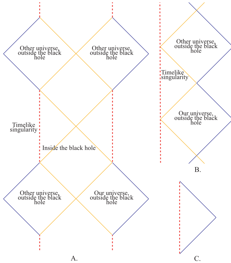
Figure 3: A. Reissner-Nordström black holes with e^2 < m^2 . B. Extremal Reissner-Nordström black holes ( e^2 = m^2 ). C. Naked Reissner-Nordström black holes ( e^2 > m^2 ).
