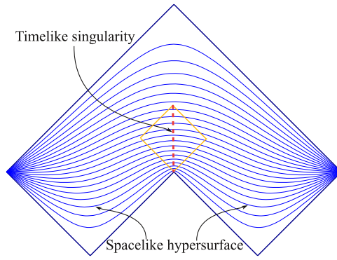
Figure 12: Primordial evaporating black hole with time-like singularity.
