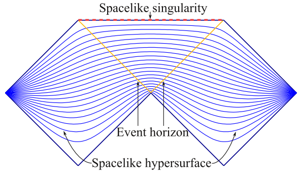
Figure 4: Space-like foliation of the maximally extended Schwarzschild solution.
