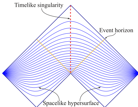
Figure 8: Space-like foliation of the extremal Reissner-Nordström solution with e^2 = m^2 .
