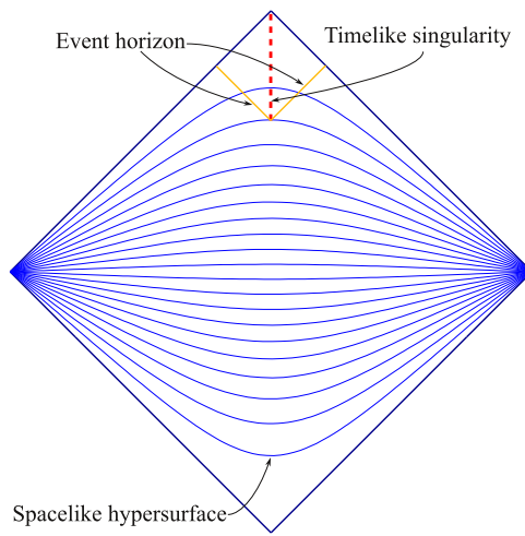
Figure 13: Non-primordial non-evaporating black hole with time-like singularity.
