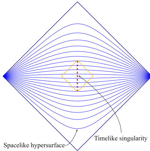
Figure 14: Non-primordial evaporating black hole with time-like singularity.
