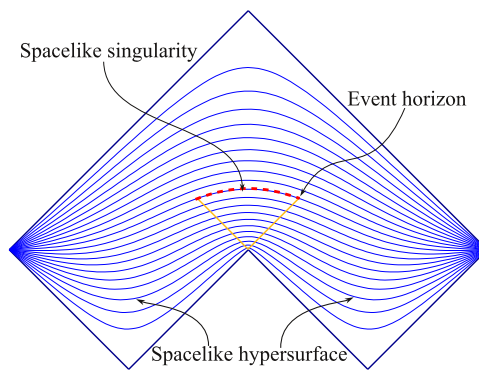
Figure 10: The space-like foliation for a primordial, non-eternal black hole with space-like singularity.
