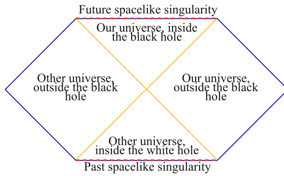
Figure 2: The maximally extended Schwarzschild solution, in Penrose coordinates.
