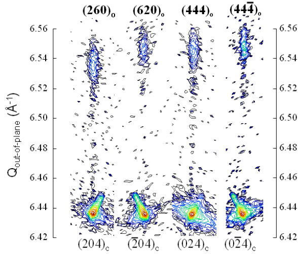
Figure 4. Room temperature XRD RLMs around the (260)_O , (444)_O , (620)_O and (444)_O reflections of a 40 nm LSMO film grown on STO.
